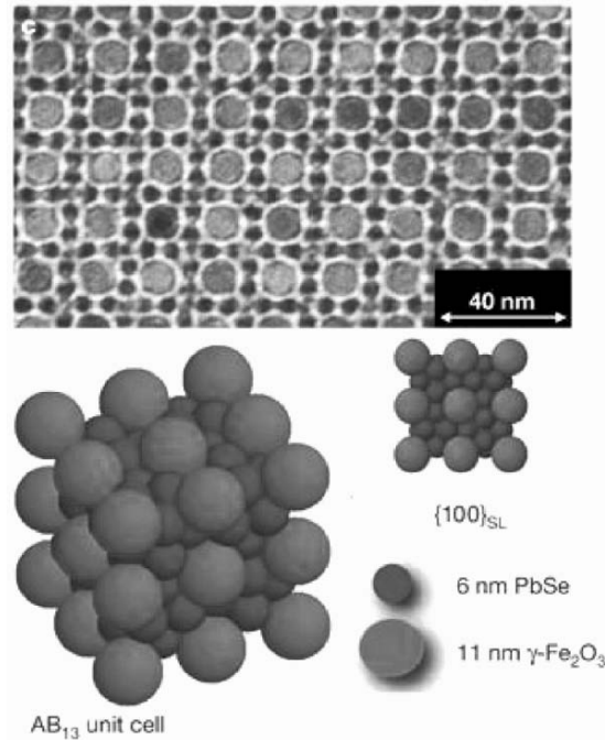
Fig. 3.12. TEM image showing a superlattice of PbSe and \gamma\text{-Fe}_2\text{O}_3 nanocrystals. The projection corresponds to \langle 100 \rangle plane of the \text{AB}_{13} structure. The \text{AB}_{13} lattice and the structure of the \langle 100 \rangle plane are illustrated (reproduced with permission from [608])
