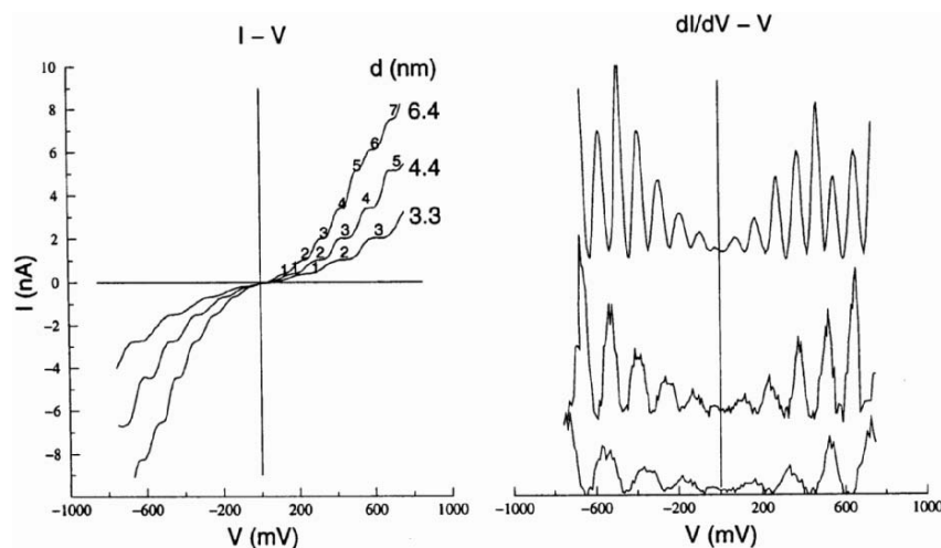
Fig. 4.8. I-V spectra of isolated PVP capped Pd nanocrystals of different diameters exhibiting Coulomb staircase behavior. The derivative spectra ( dI/dV vs. V ) are shown alongside (reproduced with permission from [678])
