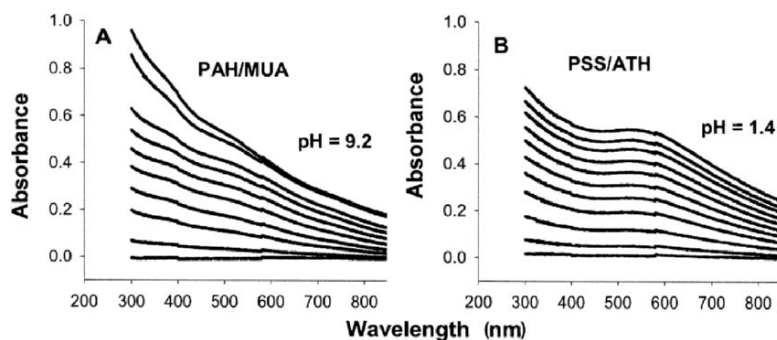
Fig. 3.18. UV–vis spectra showing layer-by-layer growth of polymer/Au nanocrystals on thiol-functionalized glass slides. (a) PAH/mercaptoundecanoic acid multilayer film formed by alternately exposing the slide to a solution of poly(allylamine hydrochloride) and another solution of a Au nanocrystals with a mixed ligand shell consisting of hexanethiol and mercaptoundecanoic acid. (b) PSS/ATH multilayer film formed by alternately exposing the slide to a solution of poly(styrene sulfonic acid) and another solution of Au nanocrystals with a mixed ligand shell consisting of hexanethiol and 4-mercaptophenylamine (ATH) (reproduced with permission from [630])
