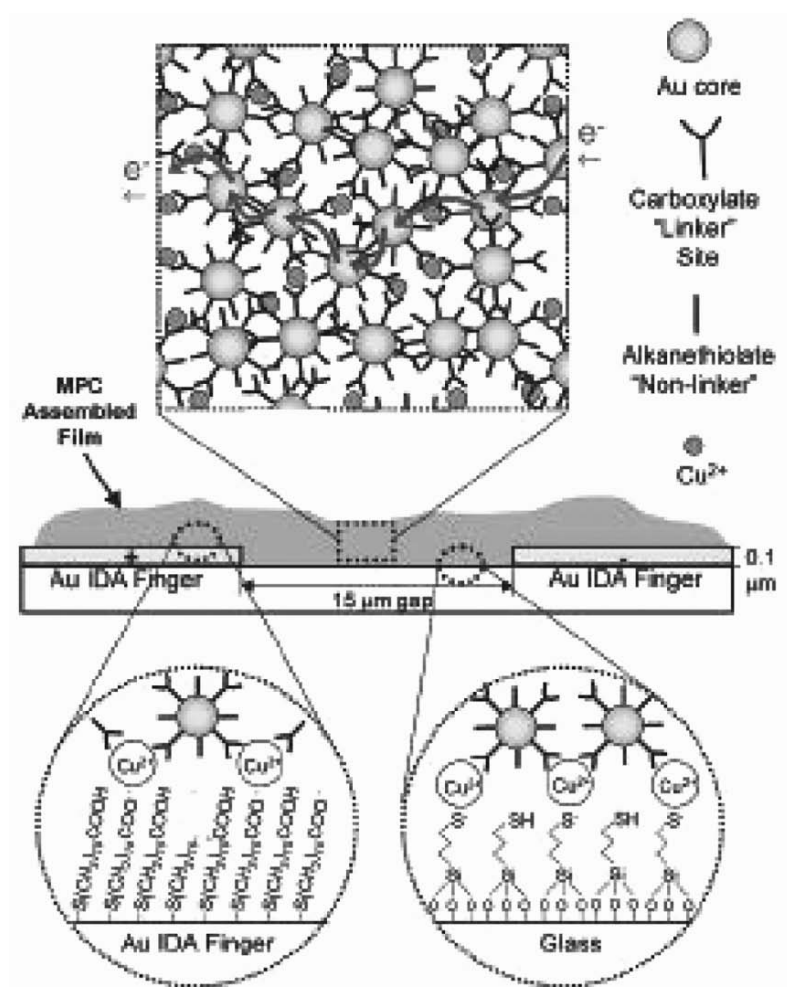
Fig. 6.13. Schematic illustration of a sensor element used to obtain the electrical response (reproduced with permission from [955])
